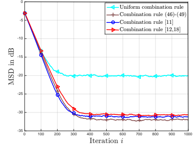
Fig. 3. Network MSD for different combination rules (close tasks).
