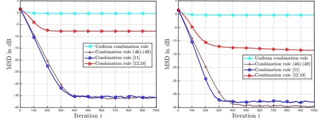
Fig. 4. Network MSD for different combination rules (distant tasks) with perfect (left) and imperfect (right) information exchange.
